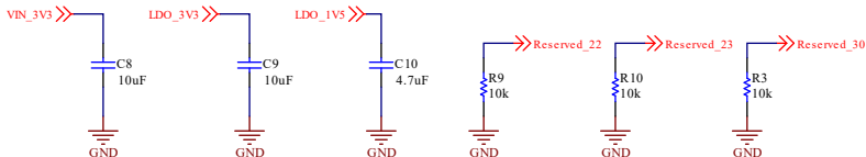
Figure 9-4. TPS25730S Sink Example Schematic
